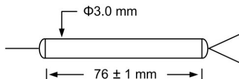
900 μm loose tube
